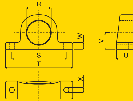
FOOT MOUNT
